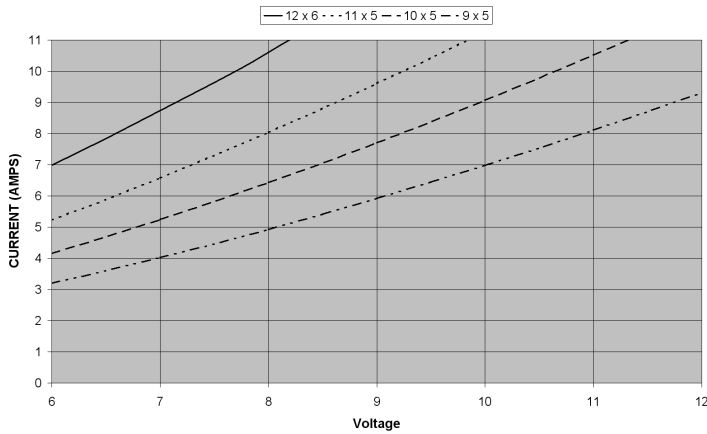
HC2808-0860 Current vs. Voltage with propeller
