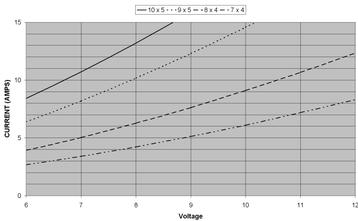
HC2808-1160 Current vs. Voltage with propeller
