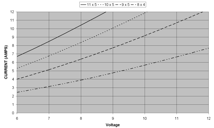
HC2808-0980 Current vs. Voltage with propeller
