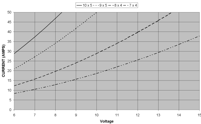
HB3630-1500 Current vs. Voltage with propeller
