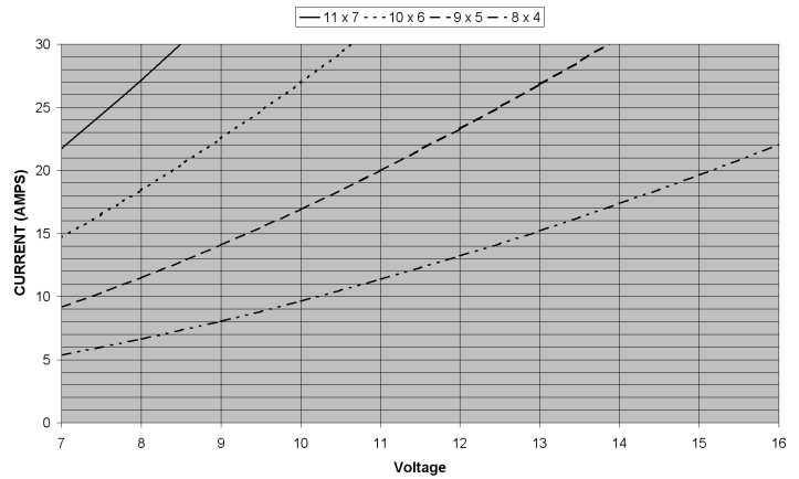
HB3630-1000 Current vs. Voltage with propeller
