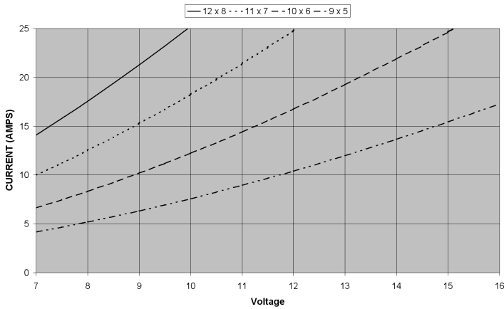
HB3630-0780 Current vs. Voltage with propeller
