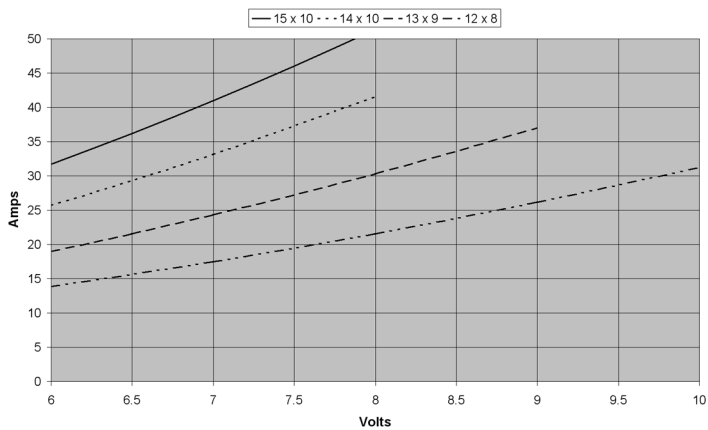
HB3615-3243 Current vs. Voltage with Propeller
