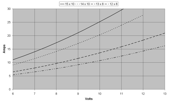
HB3615-2143 Current vs. Voltage with Propeller
