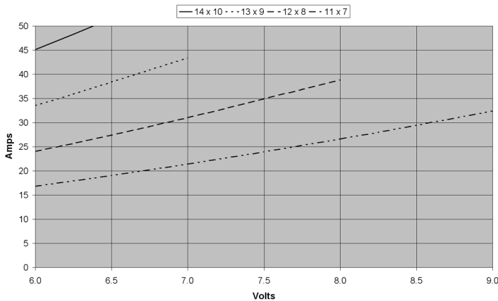
HB3615-3233 Current vs. Voltage with Propeller
