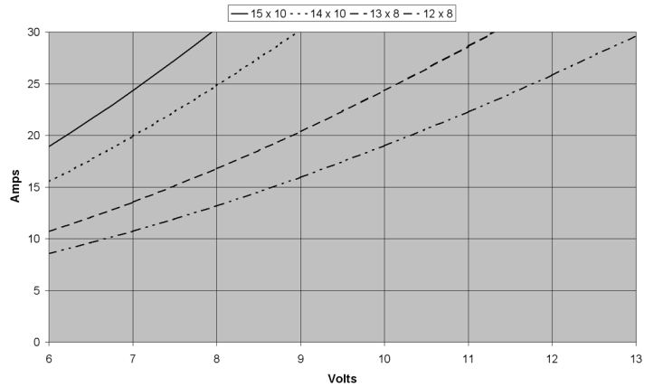
HB3615-2133 Current vs. Voltage with Propeller
