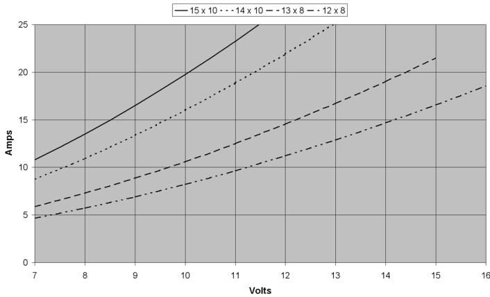
HB3615-1633 Current vs. Voltage with Propeller
