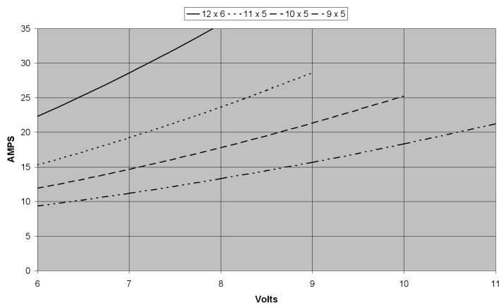
HB2815-4043 Current vs. Volts with propeller
