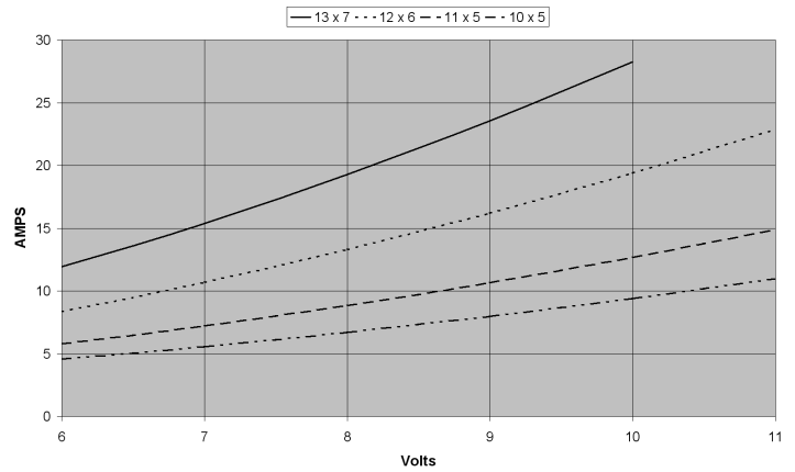
HB2815-3043 Current vs. Volts with propeller
