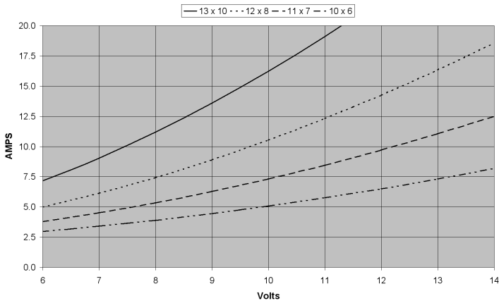
HB2815-2043 Current vs. Volts with propeller
