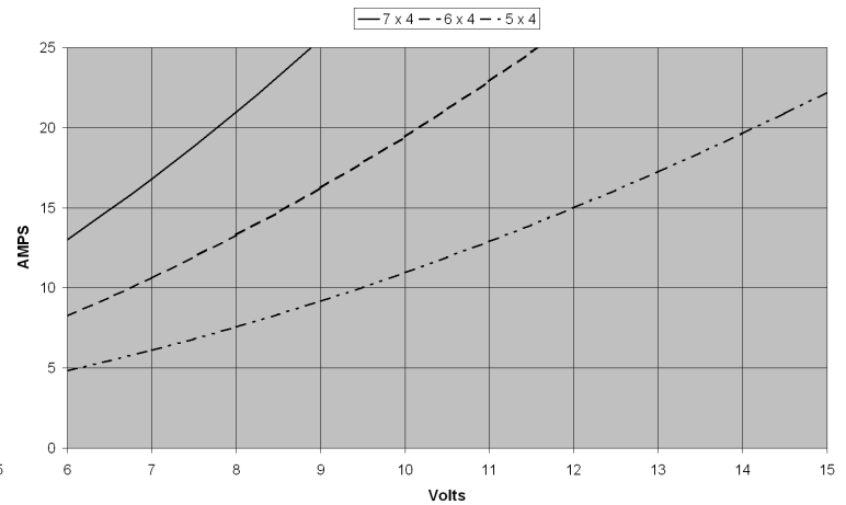
HB2815-2000 Current vs. Volts with propeller
