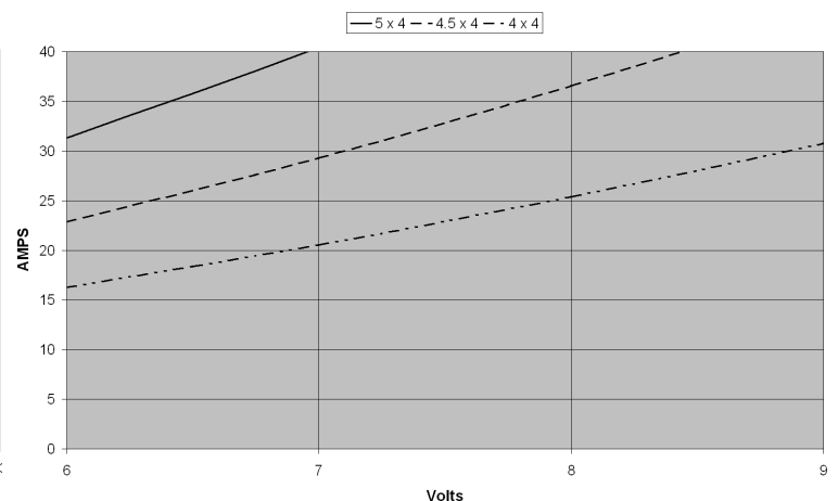
HB2815-4000 Current vs. Volts with propeller
