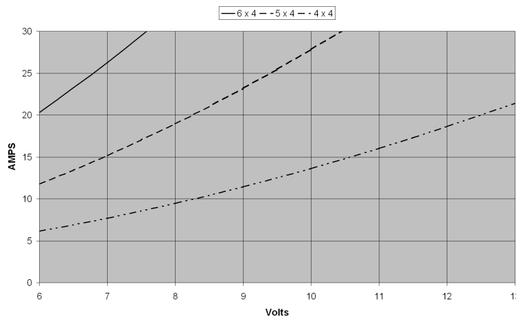
HB2815-3000 Current vs. Volts with propeller
