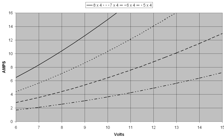
HB2815-1400 Current vs. Volts with propeller
