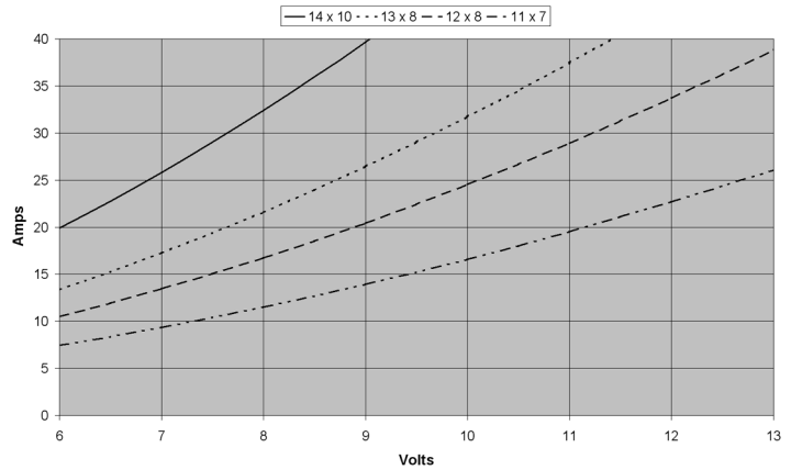
HA3618-3043 Current vs. Voltage with Propeller
