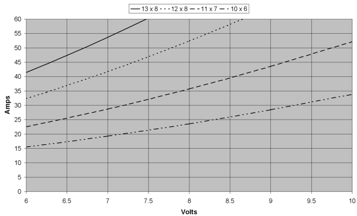
HA3618-4543 Current vs. Voltage with Propeller
