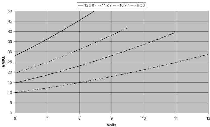
HA2825-4443 Current vs. Volts with propeller
