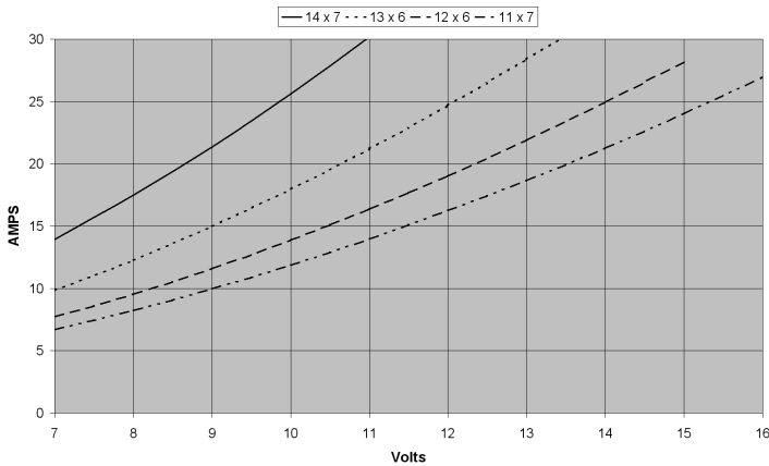
HA2825-2743 Current vs. Volts with propeller
