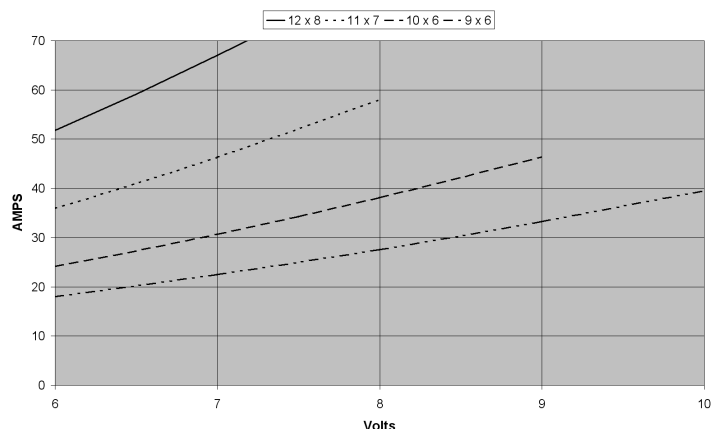
HA2825-5543 Current vs. Volts with propeller
