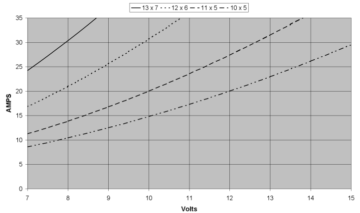
HA2825-3643 Current vs. Volts with propeller
