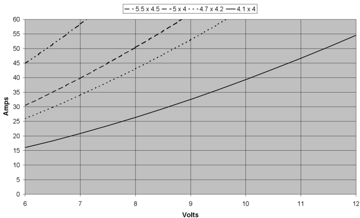
HA2825-4400 Current vs. Voltage with Propeller
