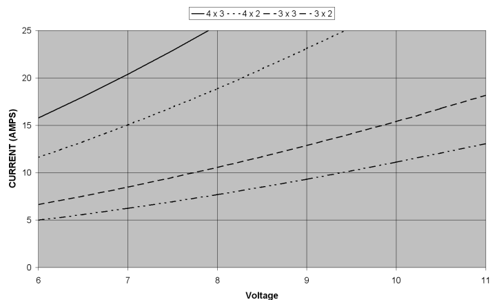
HA2025-5300 Current vs. Voltage with propeller
