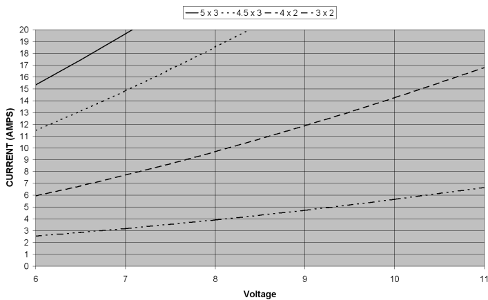
HA2025-4200 Current vs. Voltage with propeller
